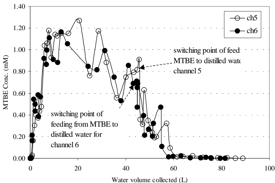
Figure 2. Comparison of the groundwater effluent concentrations from channels 5 and 6 as a function of effluent water volume. Both channels were planted with alfalfa plants and were inoculated with strain #41 ( Arthrobacter ), but ch6 was aerated while ch5 was not.
