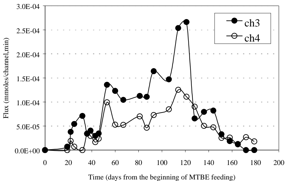
Figure 6. Gas flux from channels 3 and 4 as a function of days from the beginning of MTBE feeding. Neither channel was inoculated with any additional strain. Channel 3 was planted while channel 4 was not. The feeding was switched from MTBE to distilled water on the 83rd day.
