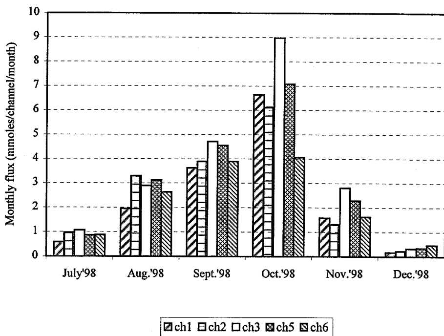
Figure 8. Channel soil gas flux of MTBE for each month for the planted channels.
